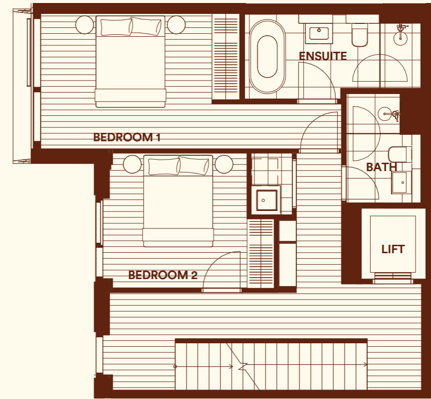
LEVEL 01
