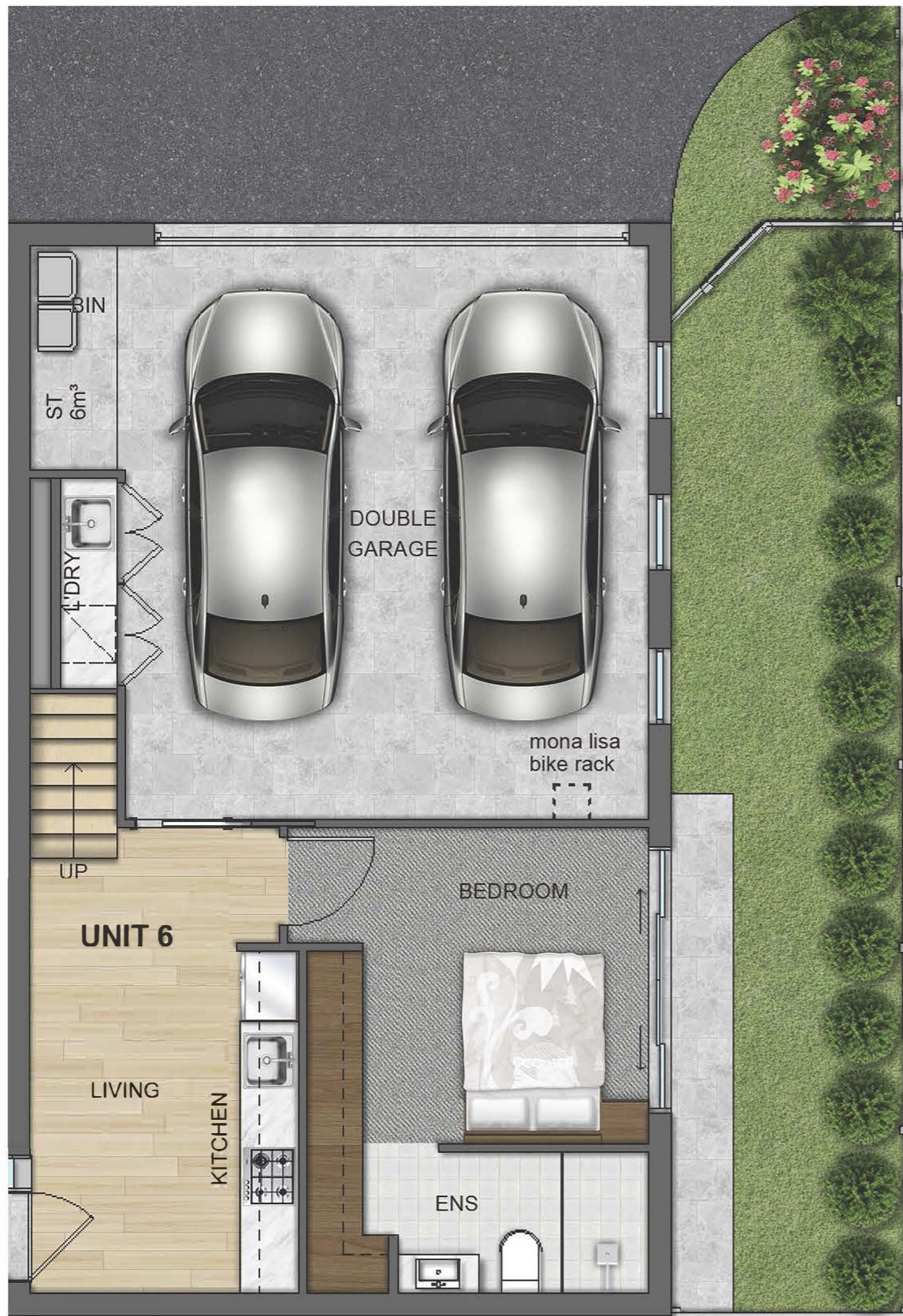
GROUND FLOOR
