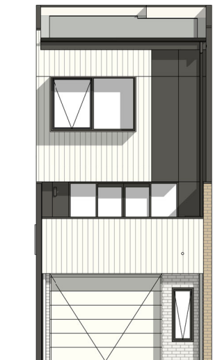
REAR ELEVATION - NTS
