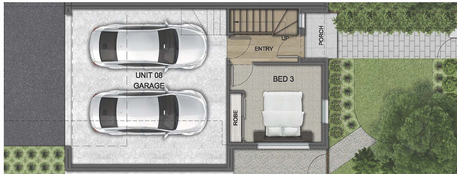
GROUND FLOOR
