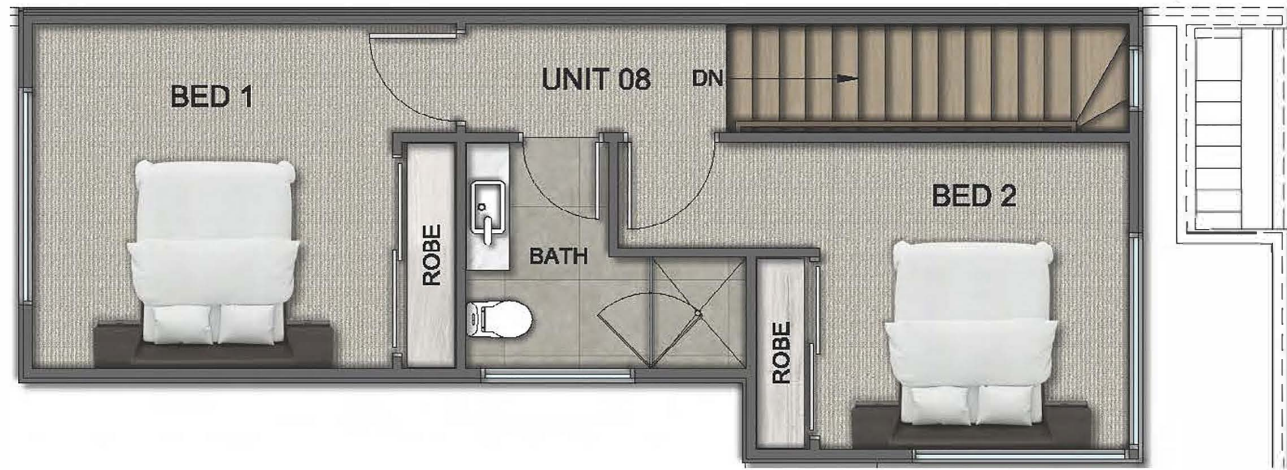
SECOND FLOOR
