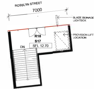
1 R18 - UPPER LEVEL
