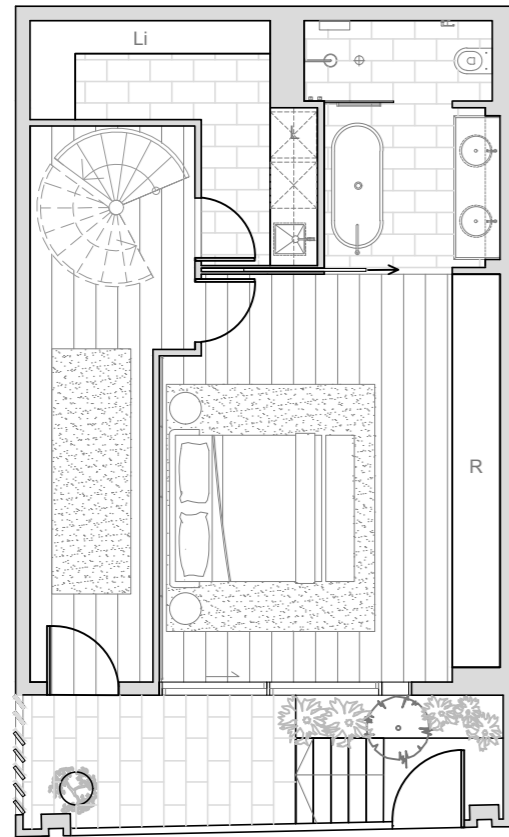
GROUND FLOOR LEVEL
